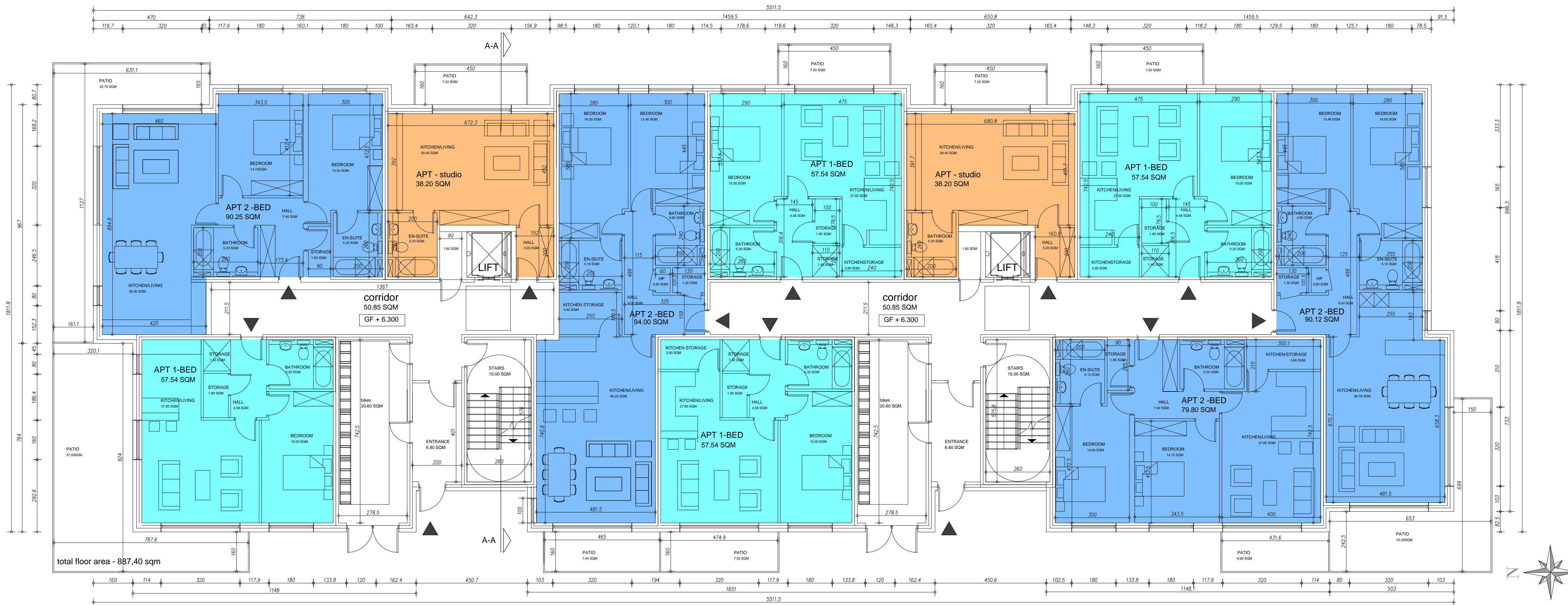
1 PROPOSED BLOCK 5 - GROUND FLOOR PLAN 1:100
