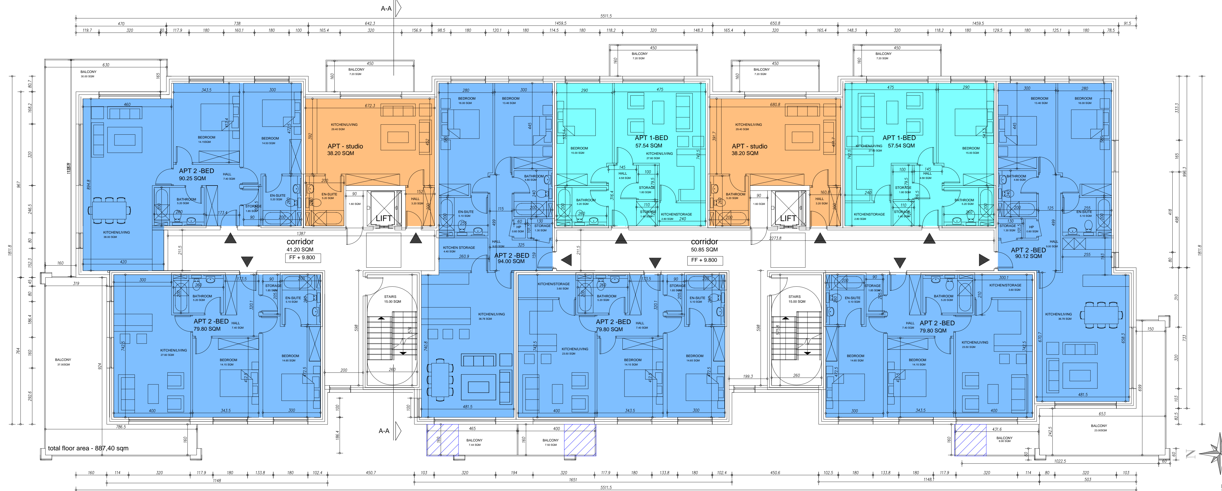
1 PROPOSED BLOCK 5 - 1st-5th FLOOR PLAN 1:100
